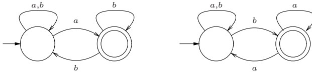
Fig. 1. An NBW for “at last one a and at least one b ”
