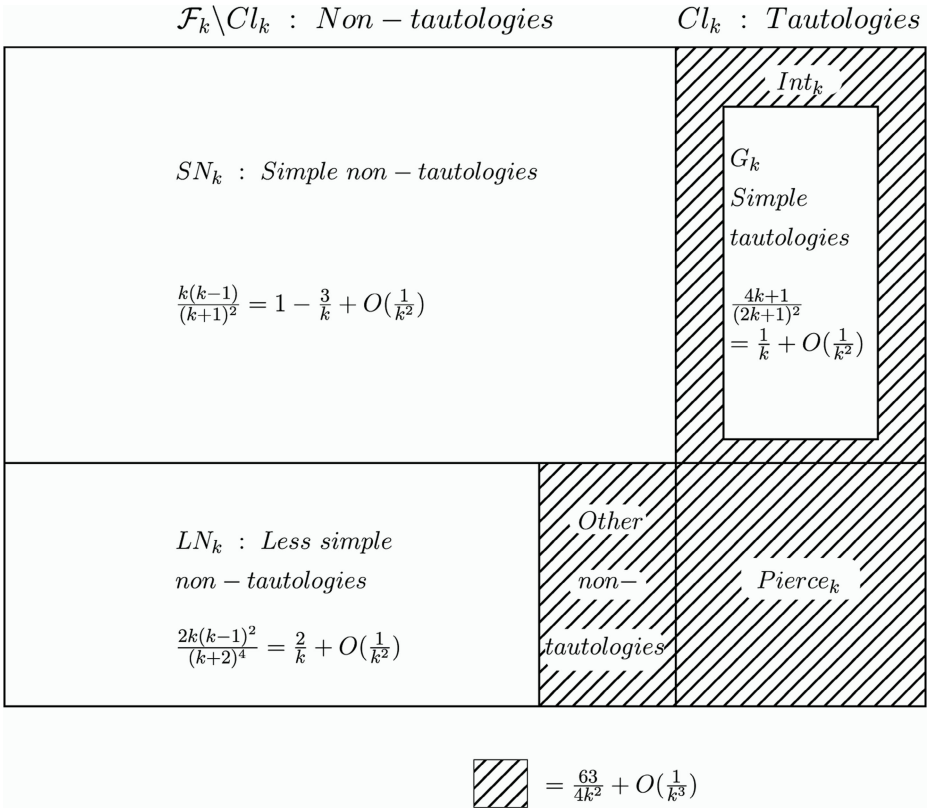
Fig. 2. Densities of simple tautologies, simple and less simple non-tautologies
