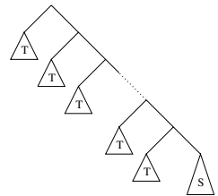
Fig. 2. A tree with T \neq S
