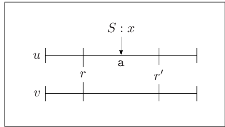
Fig. 6. A letter \mathbf{a} occurs between n -rankers r, r' in u but not in v
